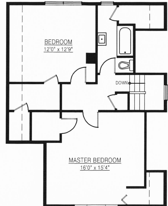
UPPER FLOOR PLAN FLOOR AREA: 671 sq.ft. UNDER 4' AREA: 93 sq.ft.
