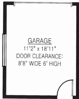
GARAGE FLOOR PLAN FLOOR AREA: 243 sq.ft..
